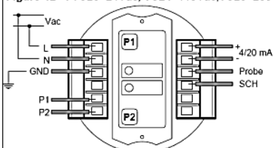
Figure 4B : TC23=24Vac, TC24=115Vac,TC25=230Vac
