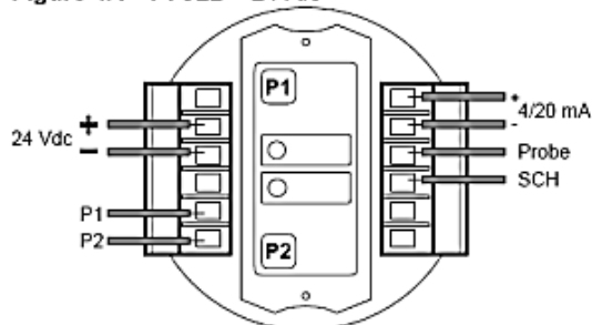
Figure 4A : TC22 = 24Vdc
